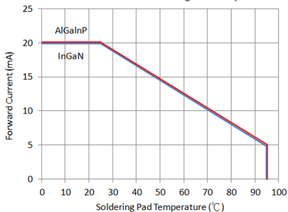
Forward Current vs. Soldering Pad Temperature
